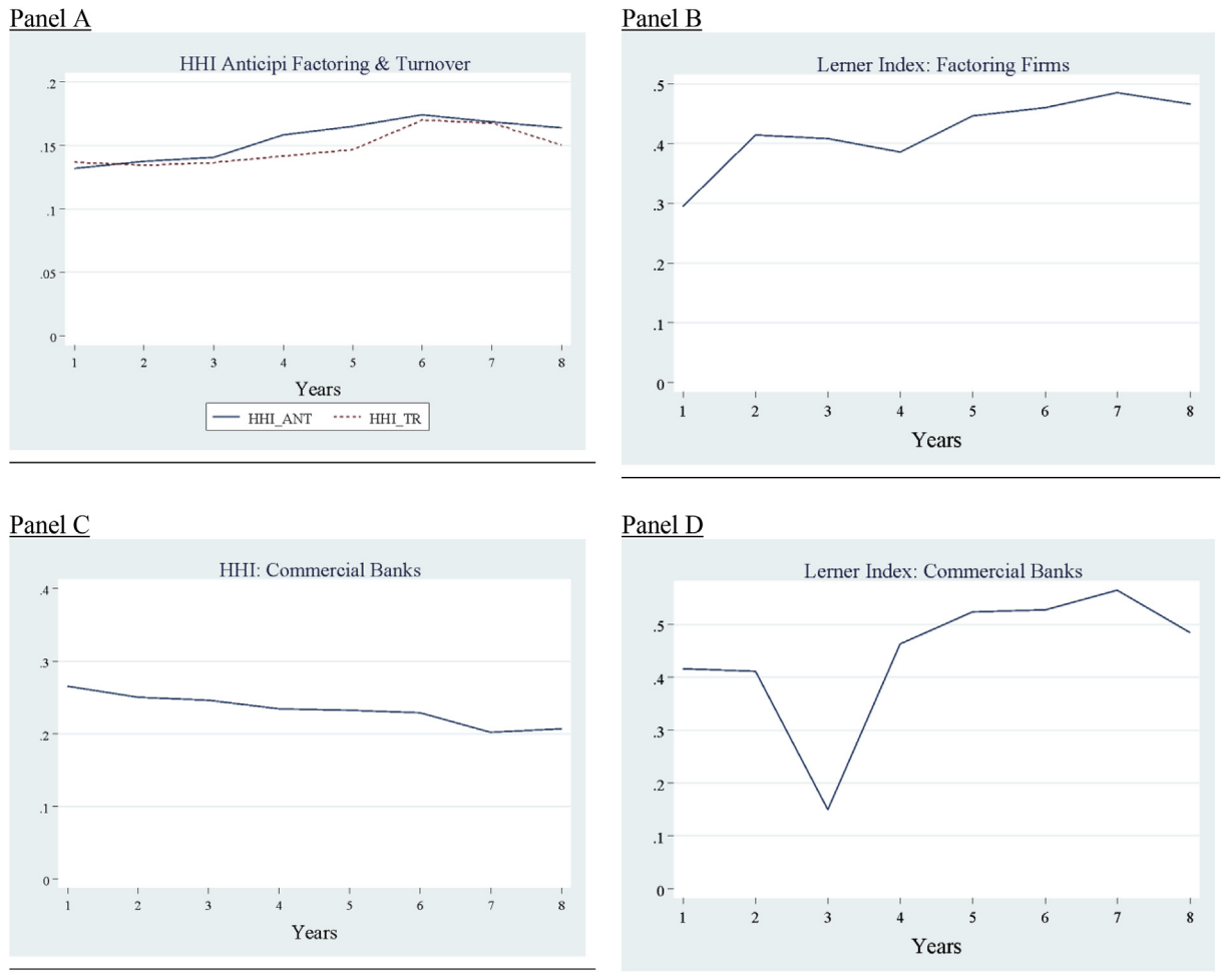
Fig. 1. The evolution of competition indicators in the Factoring industry. This figure reports the evolution of competition and stability indicators in the factoring industry over time. Specifically, we report the Herfindahl-Hirschman Index for factoring companies (panel A: top left), measured with the outstanding value of trade credits at the end of the year (HHI-ANT) and the overall value of all trade credits in the year (HHI-TR). In the panel B (top-left), we report the Lerner index for factoring companies. In the Panel C (down-left) and D (Down-right), we report the HHI (calculated based on total assets) and the Lerner indices for banks, respectively. In all graphs, years: 1, ...,8 correspond to years: 2008–2015.
